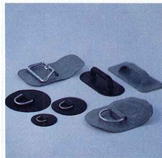
7. "D" RINGS, BOW RINGS and SAFETY/LIFT HANDLES
