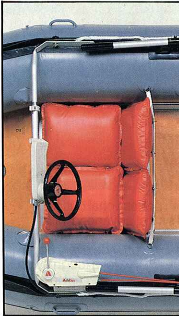
STEERING SYSTEM
