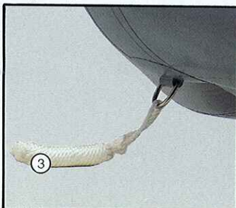
Sport Dinghies Dring and painter line.
